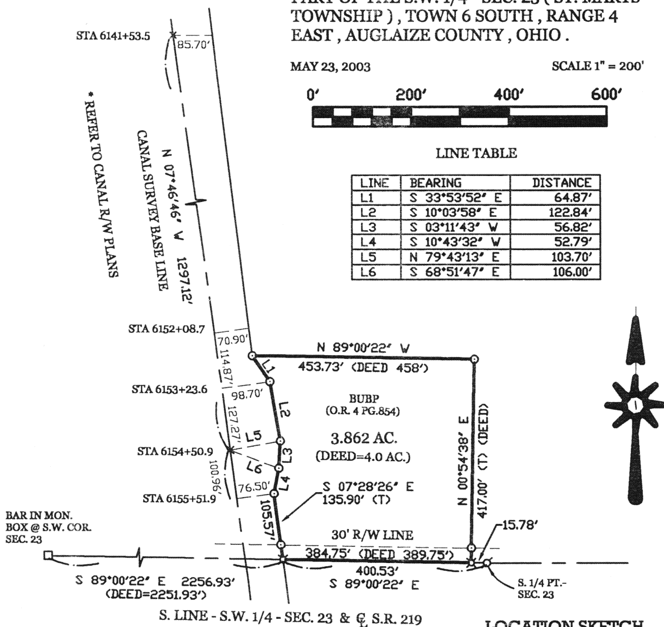
LOCATION SKETCH
