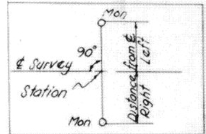
TYPICAL DETAIL FOR LOCATION OF MONUMENTS
