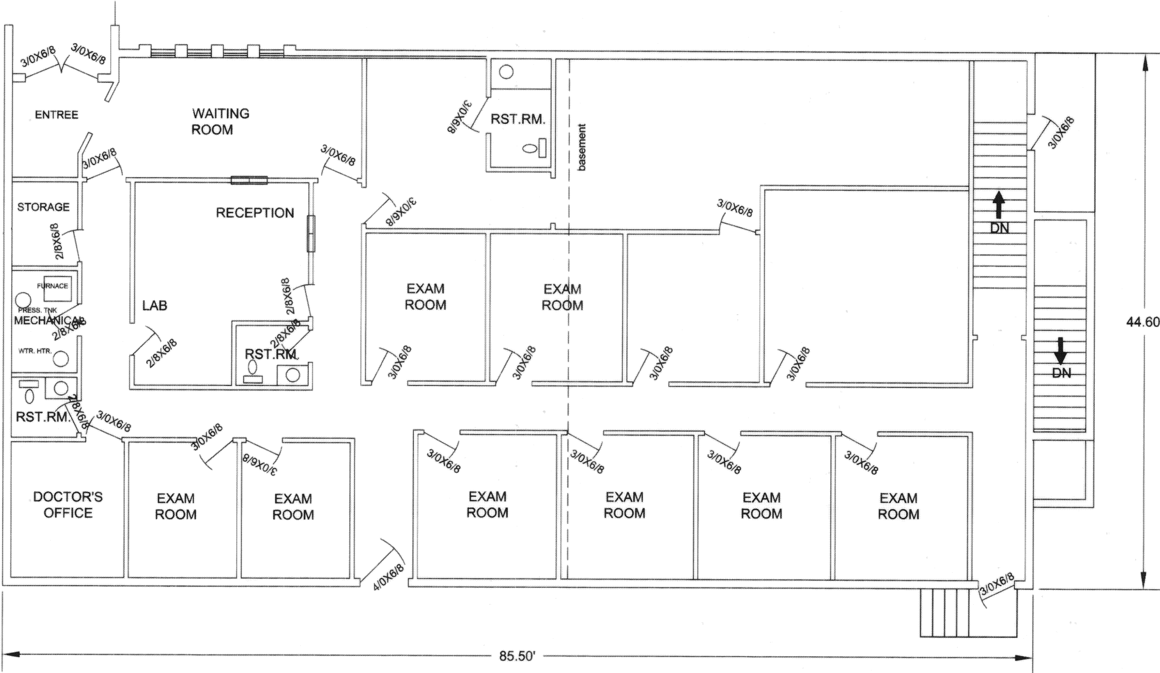
UNIT TWO FLOOR PLAN
